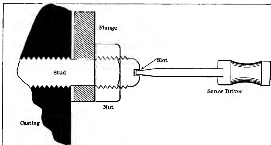
Fig. 1—A case where a stud may be fitted which can be adjusted by means of a screwdriver
